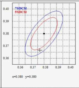
SDCM-5.6 Color Difference Chart
